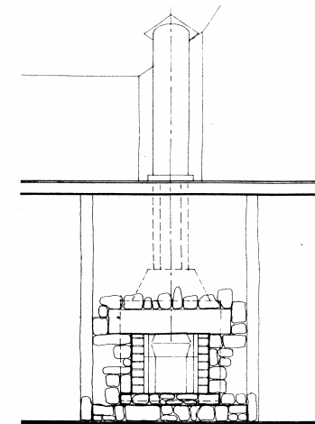
Chimney Detail
